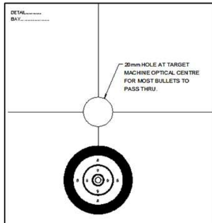
Typical offset target for 50 metre electronic machines.
